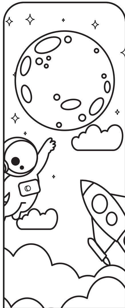
FULL MOON
