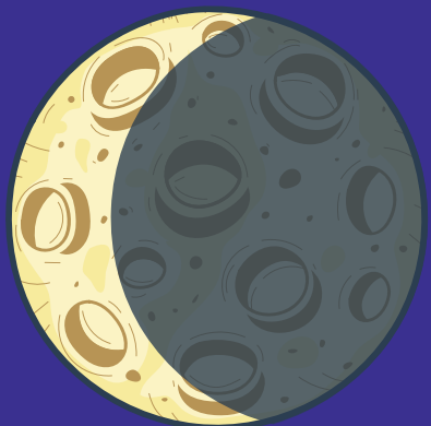
Waning Crescent
