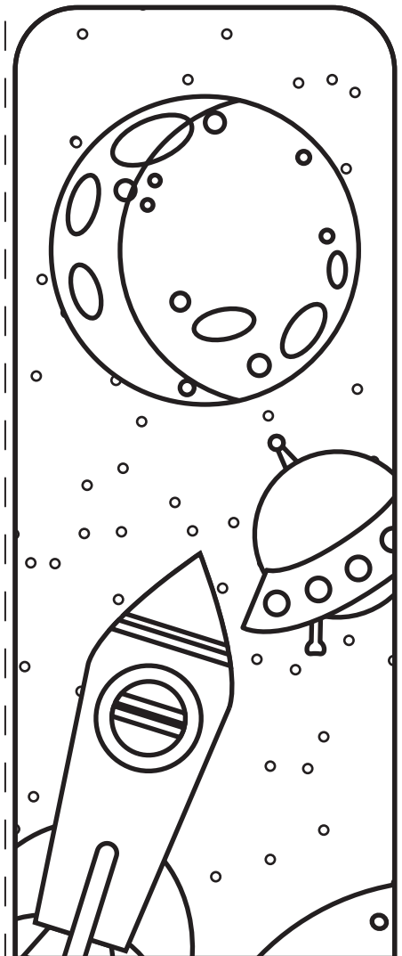
WANING CRESCENT
