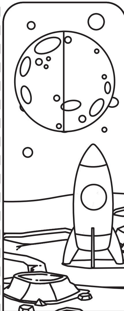
LAST QUARTER
