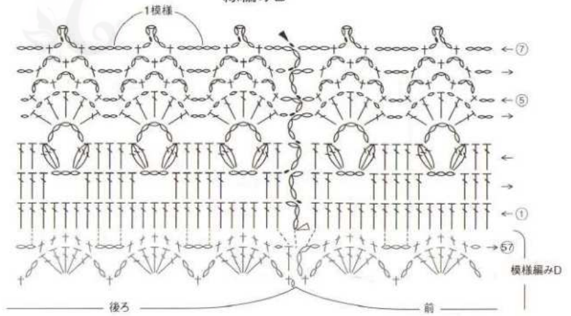
縁編みB
